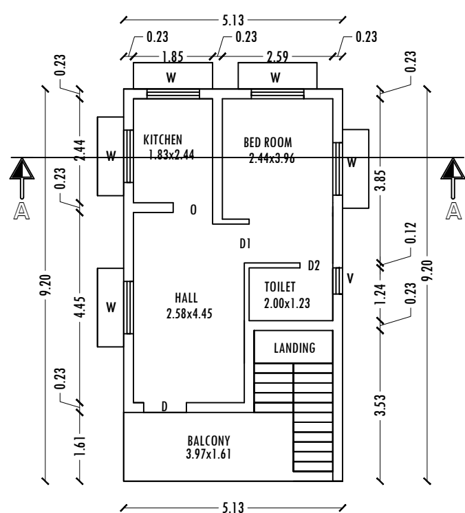
EXG. FIRST FLOOR PLAN
