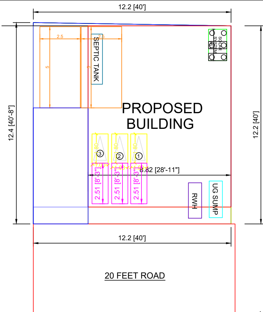
SITE PLAN SHOWN IN SHEET 2
