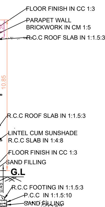
SECTION ON AB
