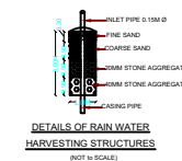
DETAILS OF RAIN WATER HARVESTING STRUCTURES
