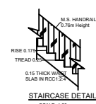
STAIRCASE DETAILS
