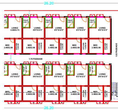
PRO-FIRST FLOOR PLAN SCALE:1:100
