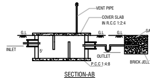
SECTION-AB
