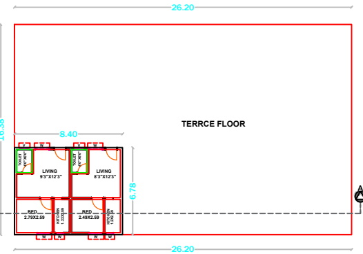
PRO-SECOND FLOOR PLAN SCALE:1:100
