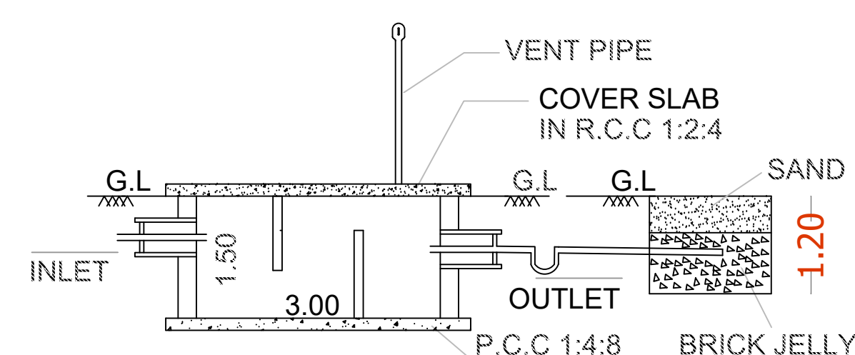
SECTION-AB
