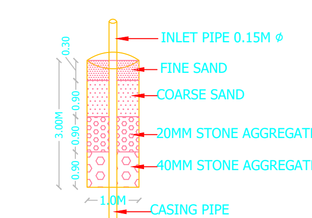
DETAILS OF RAIN WATER HARVESTING STRUCTURES (NOT to SCALE) RWH_CAPACITY_L=5000LTRS WATER_TANK_CAPACITY_L=3000LTRS
