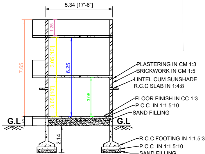
SECTION -"AB"
