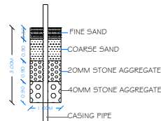
DETAILS OF RAIN WATER HARVESTING STRUCTURES
