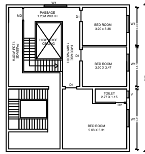
PRO.SECOND FLOOR PLAN
