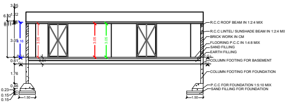
SECTION ON-AA
