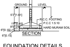
FOUNDATION DETAILS
