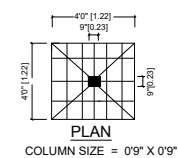
LOCATION PLAN
