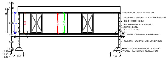
SECTION ON-AA
