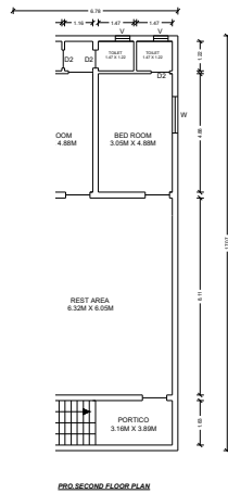
PRO. SECOND FLOOR PLAN
