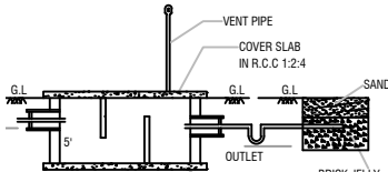
SECTION-AB
