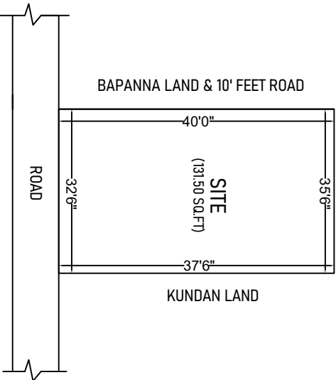
SITE DETAIL'S
