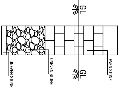
STONE FOUNDATION
