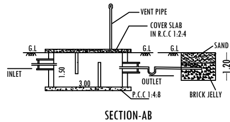
SECTION-AB
