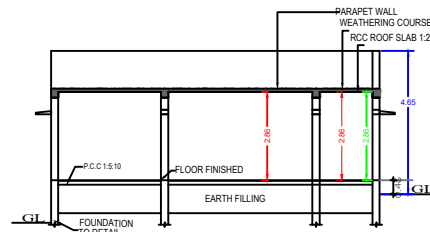
SECTION "A-B" BLOCK 1 & 2
