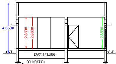
SECTION "A-B"
