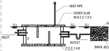
SECTION-A-B
