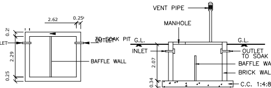
SEPTIC TANK
