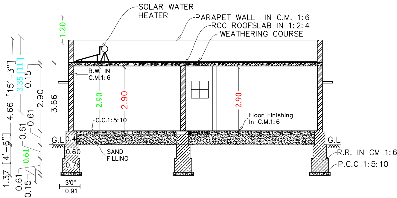
SECTION - AA
