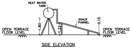
SIDE ELEVATION
