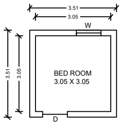
PRO. GROUND FLOOR PLAN.
