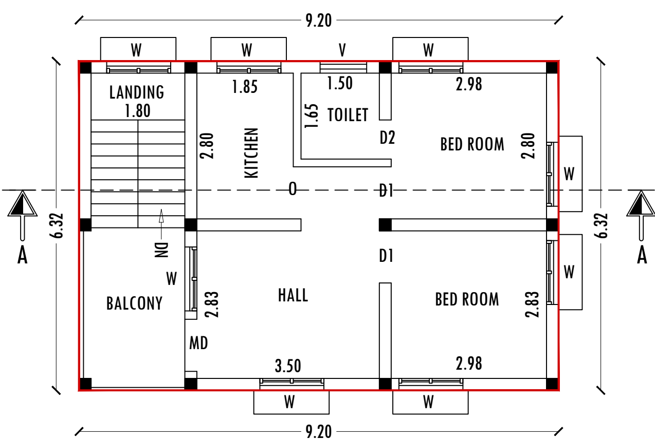
EXTG-FIRST FLOOR PLAN
