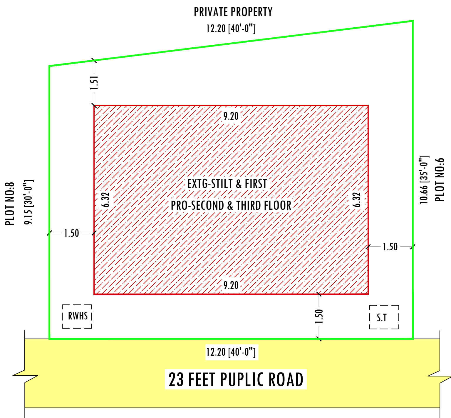
SITE PLAN
