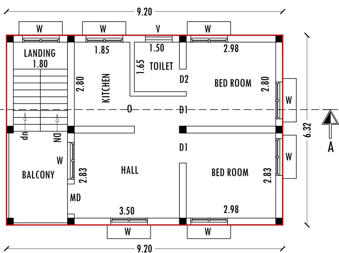
PRO-SECOND FLOOR PLAN
