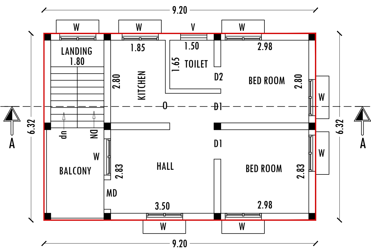
PRO-THIRD FLOOR PLAN
