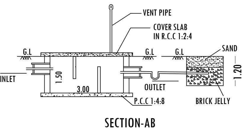
SECTION-AB
