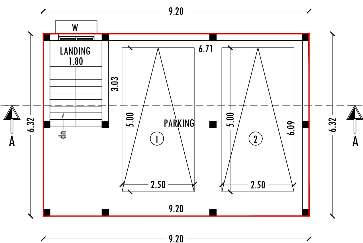
EXTG-STILT FLOOR PLAN
