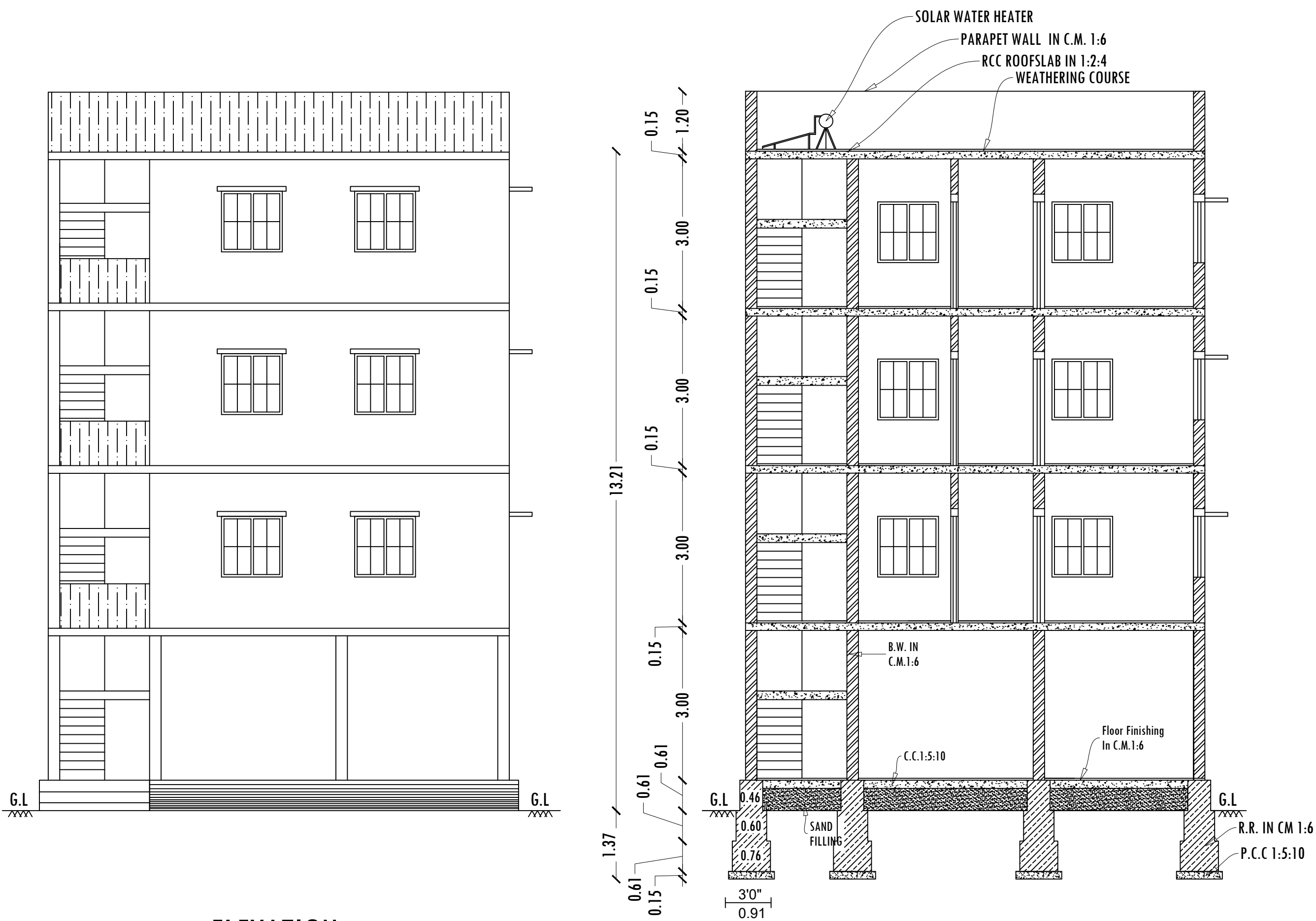
SECTION -AA
