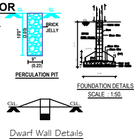
Dwarf Wall Details
