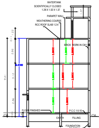
SECTION "A-B"
