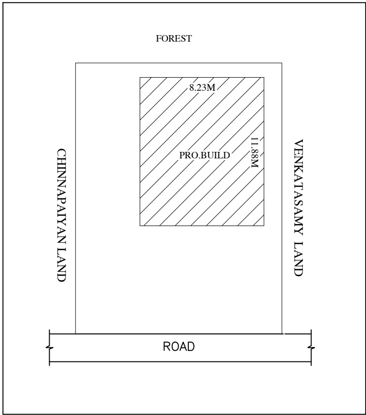
SITE PLAN
