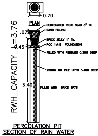
SECTION OF RAIN WATER
