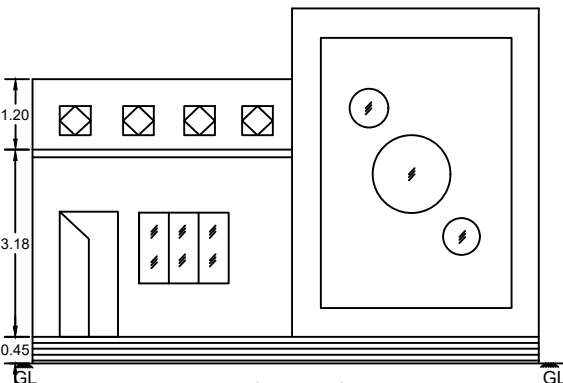
ELEVATION BY EAST
