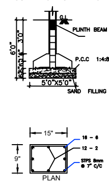
DETAILS OF COLUMN FOOTING FOUNDATION SCALE 1"=4'0"
