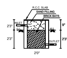
SECTION - CD
