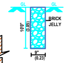
PERCOLATION PIT
