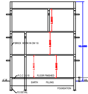
SECTION "A-B"
