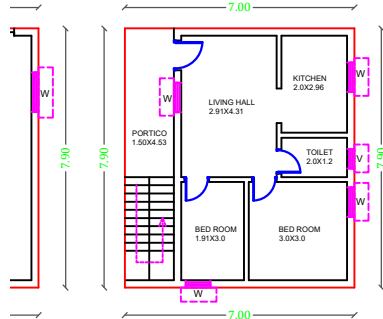
SECOND FLOOR PLAN. RESIDENTIAL
