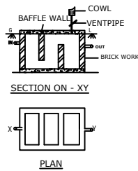
SEPTICTANK DETAILS
