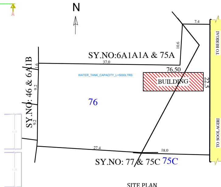
SITE PLAN
