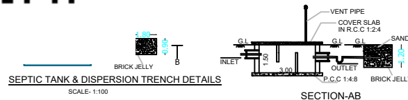
SECTION-AB
