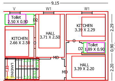
CAL FLOOR PLAN ( First floor & second floor )
