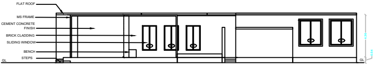
COMMUNITY CENTER ELEVATION (IN MM) SCALE-N.T.S
