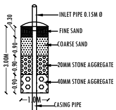
DETAILS OF RAIN WATER
