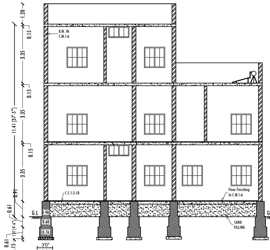
SECTION -AA
