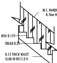
STAIRCASE DETAILS
