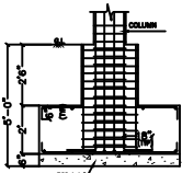
FOOTING DETAIL
