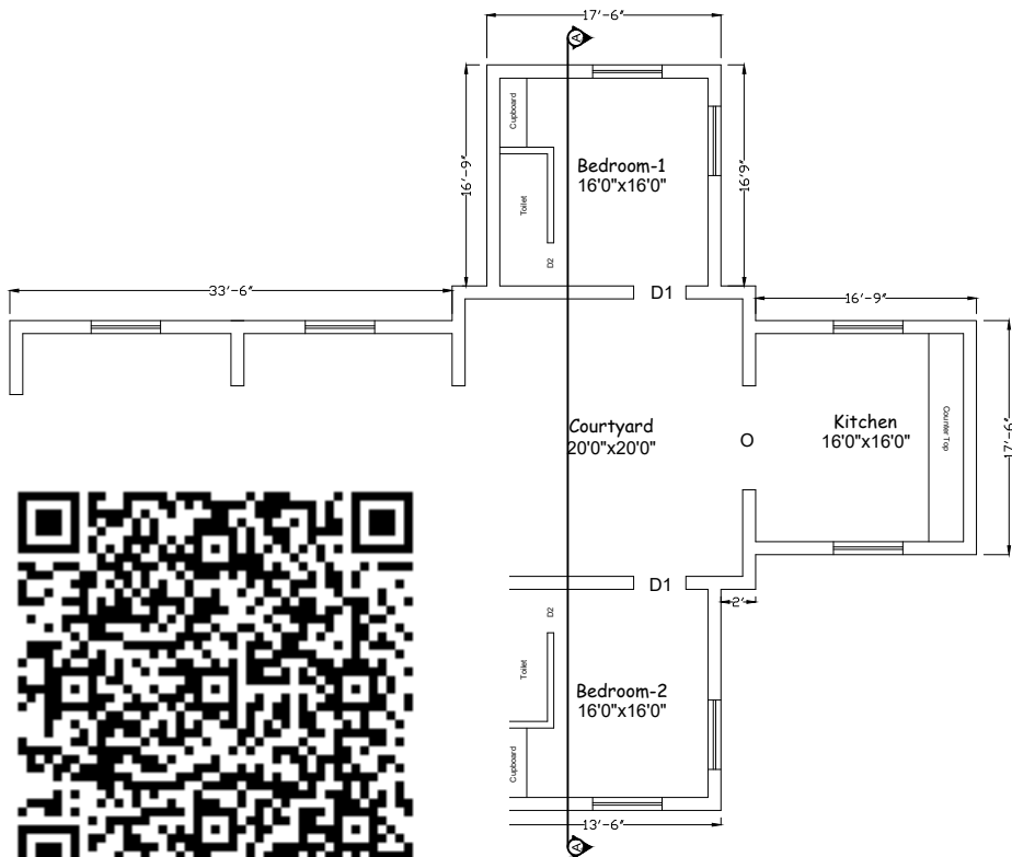
FLOOR PLAN
