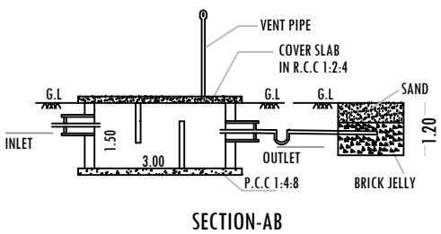
SECTION-AB
