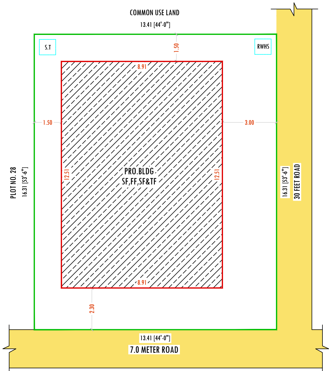
SITE PLAN
