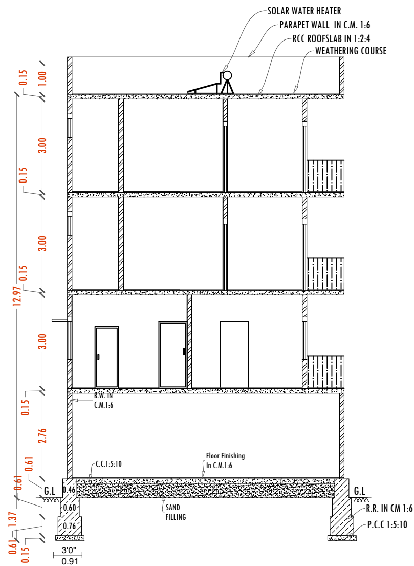
SECTION -AA
