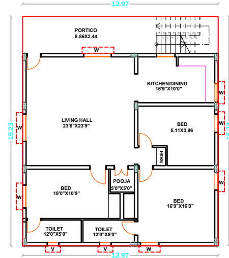
BLOCK - 2 PRO.GROUND FLOOR PLAN
