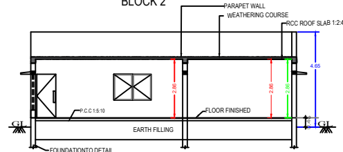
SECTION "A-B" BLOCK 2
