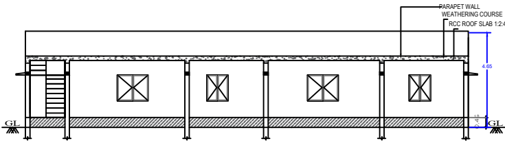
SECTION "A-B" BLOCK 1
