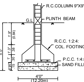
FOUNDATION DEATILS
