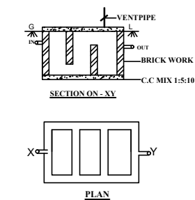
SEPTICTANK DETAILS
