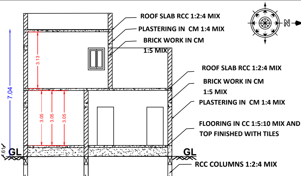
SECTION ON-AA'
