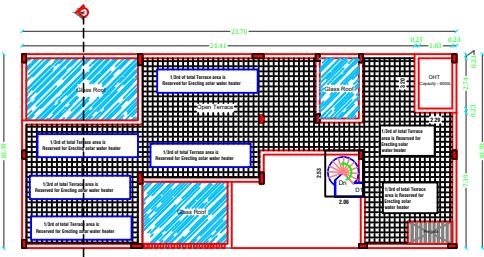
PRO. SECOND FLOOR PLAN.
