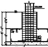
FOOTING DETAIL
