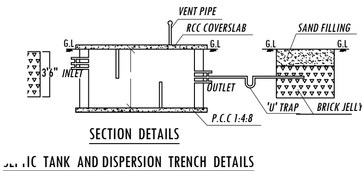
SECTION DETAILS
