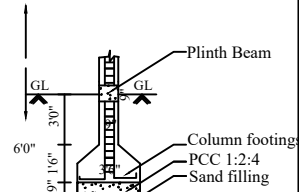
FOUNDATION DETAILS SCALE 1:50
