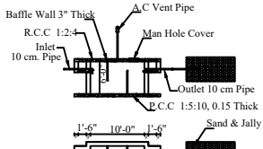
Septic Tank with Dispersion Trench
