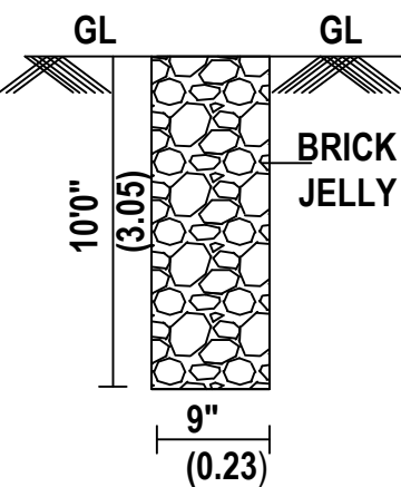
PERCOLATION PIT
