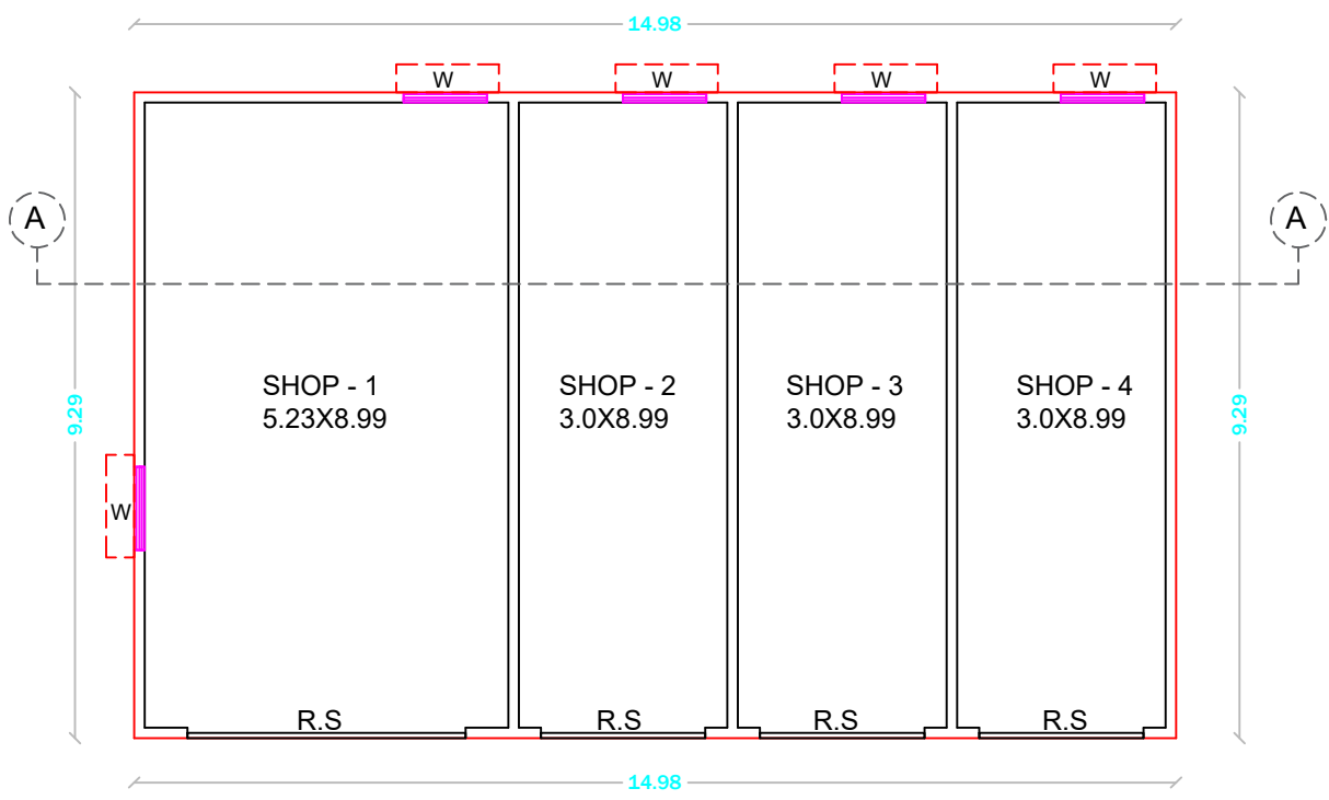
PRO.GROUND FLOOR PLAN SCALE:1:100
