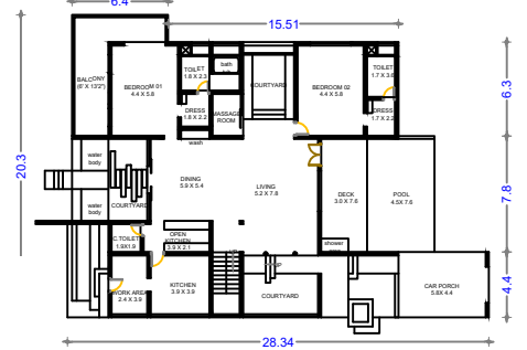
PRO. GROUND FLOOR PLAN (HOUSE 2)
