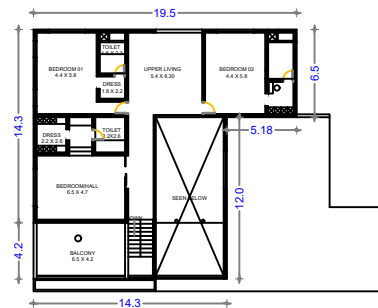
PRO. FIRST FLOOR PLAN (HOUSE 2)
