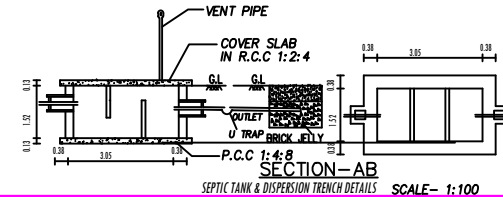
SEPTIC TANK & DISPERSION TRENCH DETAILS SCALE- 1:100
