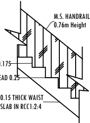
STAIRCASE DETAILS
