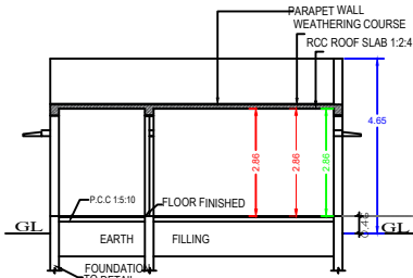
SECTION "A-B"
