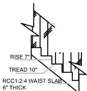
STAIRCASE DETAILS SCALE- 1:20
