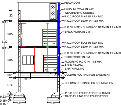
SECTION "A-B"
