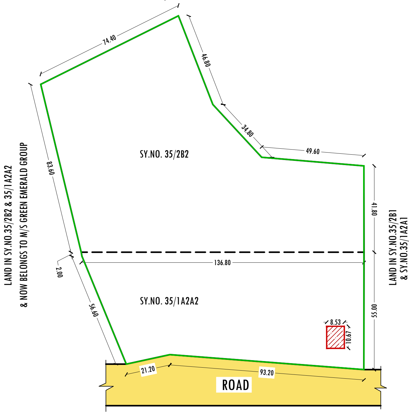
SITE PLAN SCALE- 1:1000
