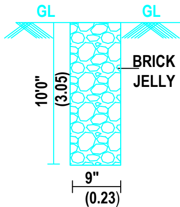
PERCOLATION PIT
