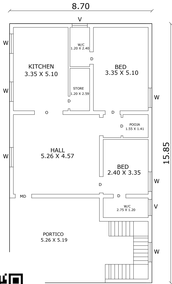
ND FLOOR PLAN
