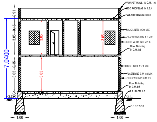
SECTION ON-"AB"
