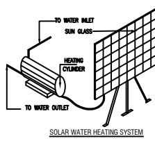
SOLAR WATER HEATING SYSTEM SCALE : 1:25
