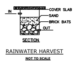
RAINWATER HARVEST NOT TO SCALE
