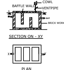
SEPTICTANK DETAILS NOT TO SCALE
