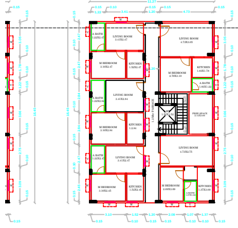
PROPOSED SECOND FLOOR PLAN
