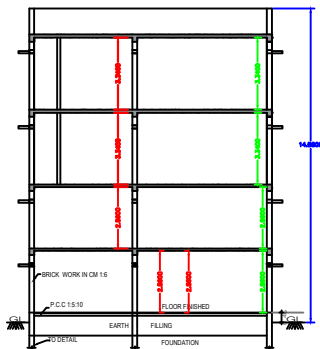
SECTION "A-B"
