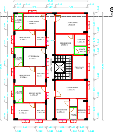
PROPOSED THIRD FLOOR PLAN
